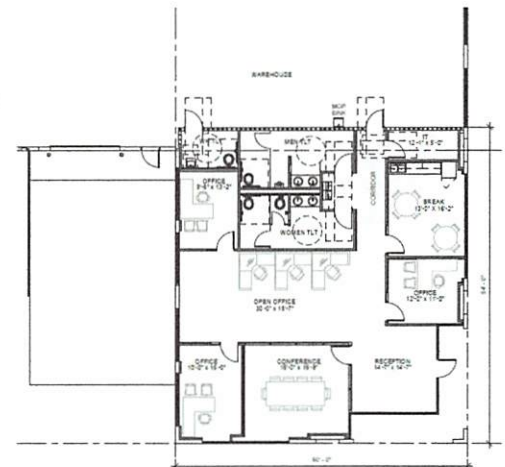
LEVEL 01 OFFICE SCHEMATIC PLAN 1/8" = 1'-0"
