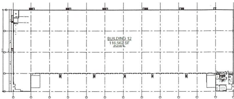
LEVEL 01 OVERALL SCHEMATIC PLAN 1/8" = 1'-0"
